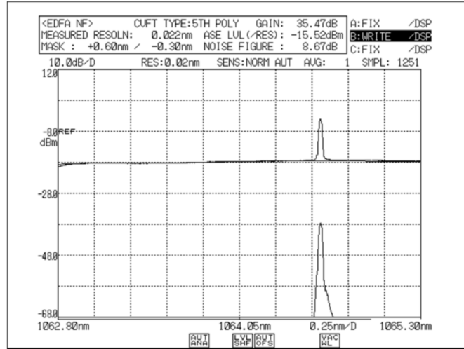
Amplified 1064 nm signal, 35 dB gain, and -3 dBm signal output power (top trace)
