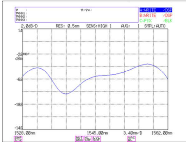
Typical Optical Spectra of ASE Output, +250C Case Temperature
